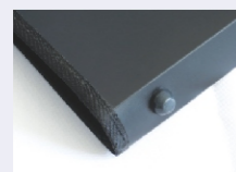
Portfolio ECS22106 Size:35*30*3.6CM ECS22107 Size:50.3*35.3*3.6CM ECS22108 Size:51*41*3.6CM ECS22109 Size:62.5*45.5*3.6CM ECS22110 Size:72*52*3.6CM ECS22111 Size:97.5*63*3.6CM ECS22112 Size:102.5*73.7*3.6CM Material:PP
